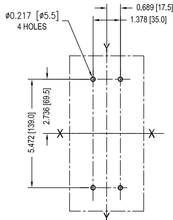
T3S 3 POLE DRILLING FRONT VIEW
