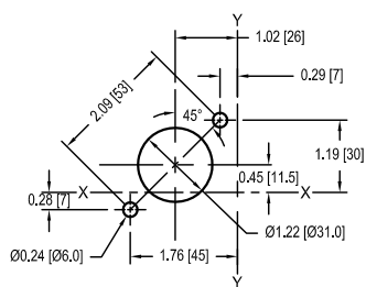
OHb HANDLE DRILLING
