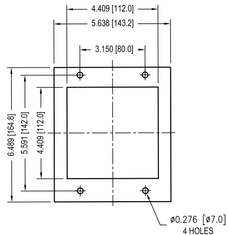
T3S 3 POLE HANDLE DOOR CUT-OUT
