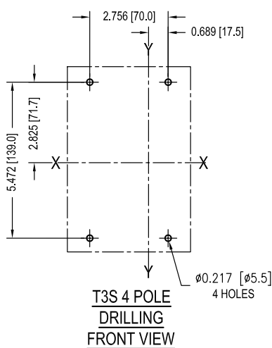
T3S 4 POLE FRONT VIEW
