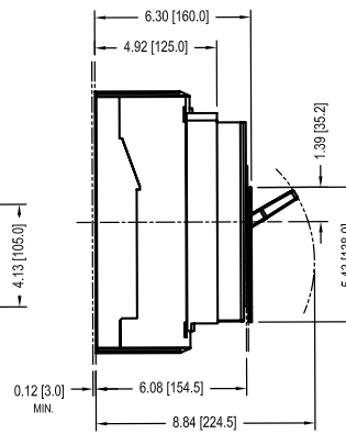
T7 3 & 4 POLE SIDE VIEW WITH REDUCED FLANGE
