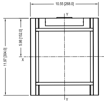
T7 3 & 4 POLE FLANGE FOR DOOR COMPARTMENT
