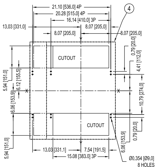
DRILLING FRONT VIEW
